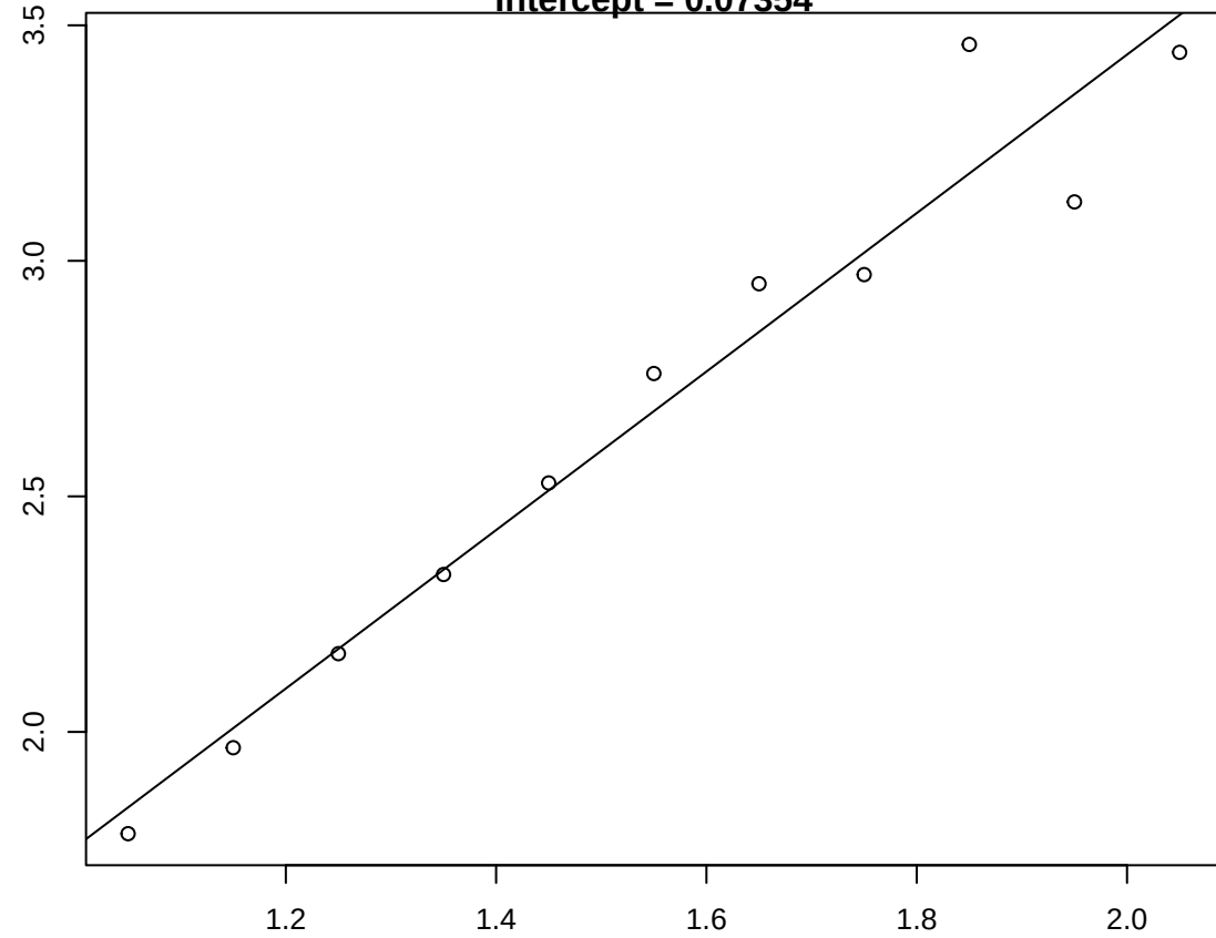
Layer 4 Intercept = 0.07354
