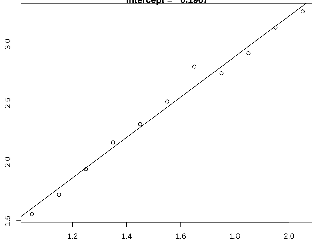
Layer 3 Intercept = -0.1967
